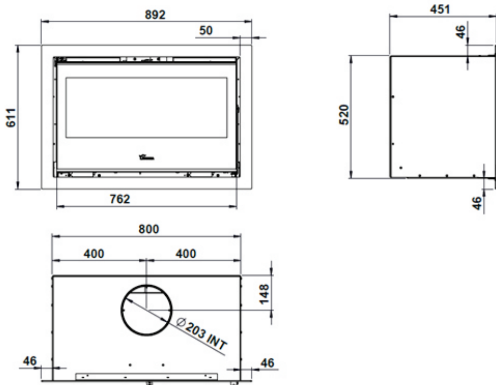
Figure No.1 - Dimensions of the SILVER 800 appliance in mm
