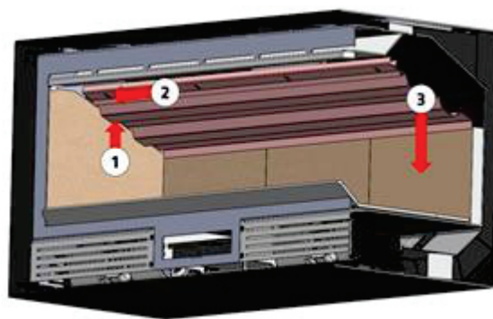
Figure No.9 - Dismantling the lower Silver deflector
