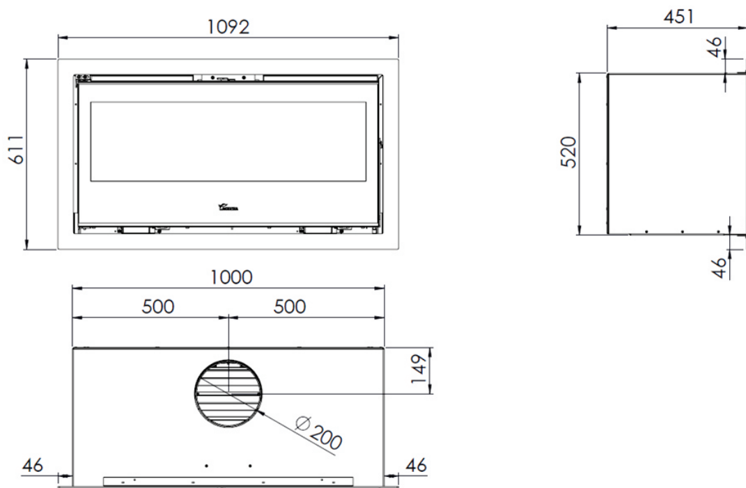
Figure No.2 - Dimensions of the SILVER 1000 appliance in mm
