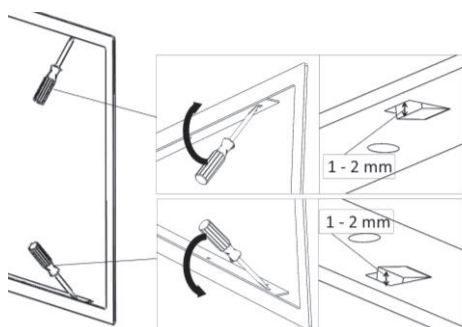
Figure No.4 - Bending the tabs
